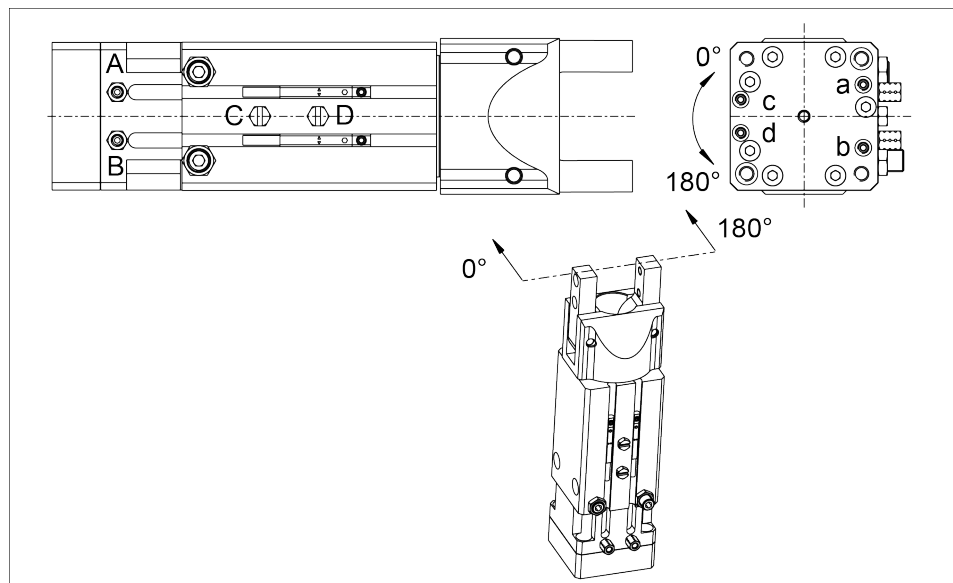
Luftanschlüsse
