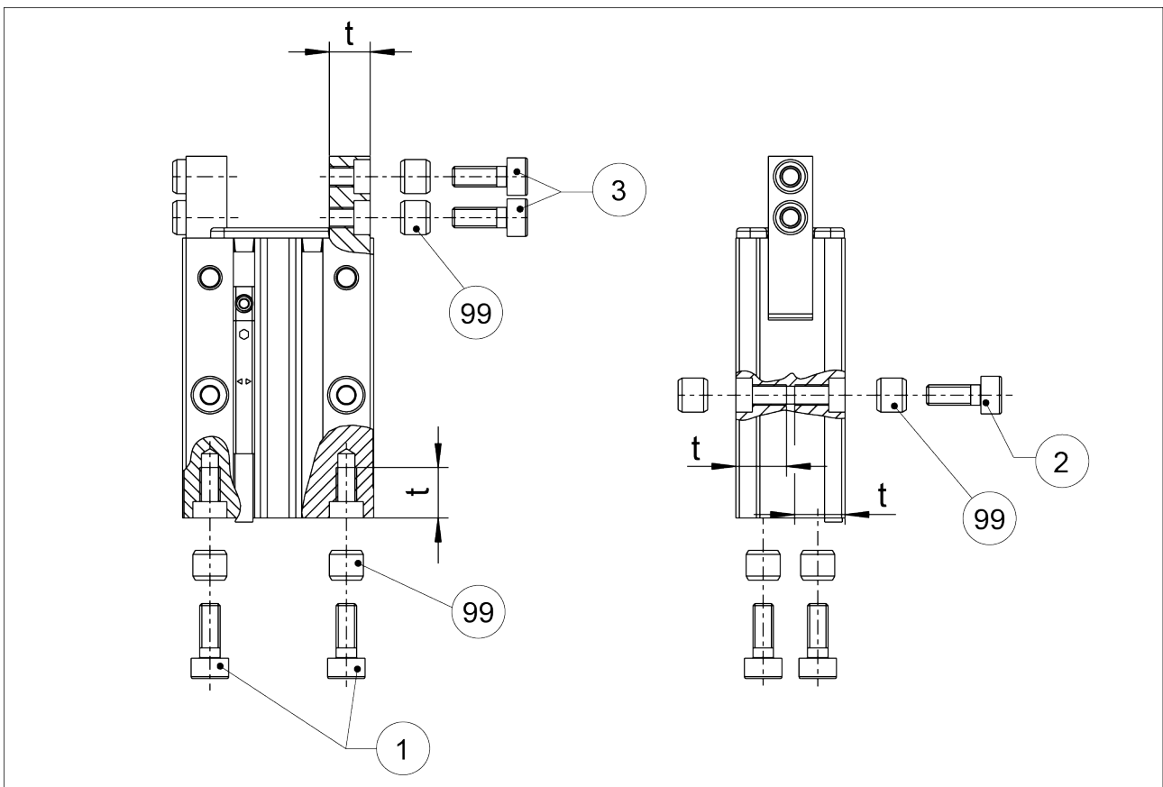
Assembly options
