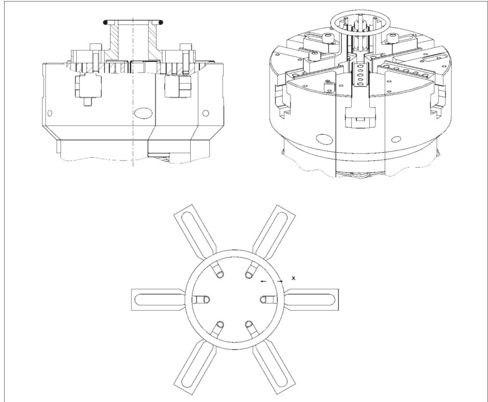
External assembly AM_1.1, Range of inside seal diameter between d_1=10 mm and d_1=60 mm
