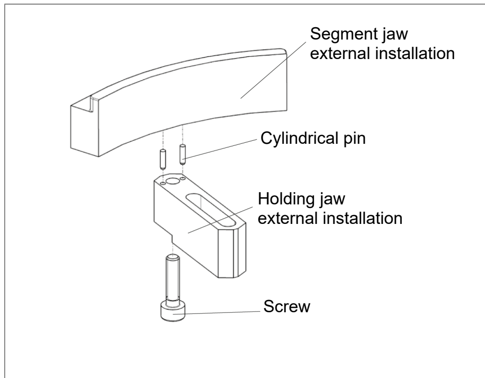
Assembly of segment jaw with clamping jaw
