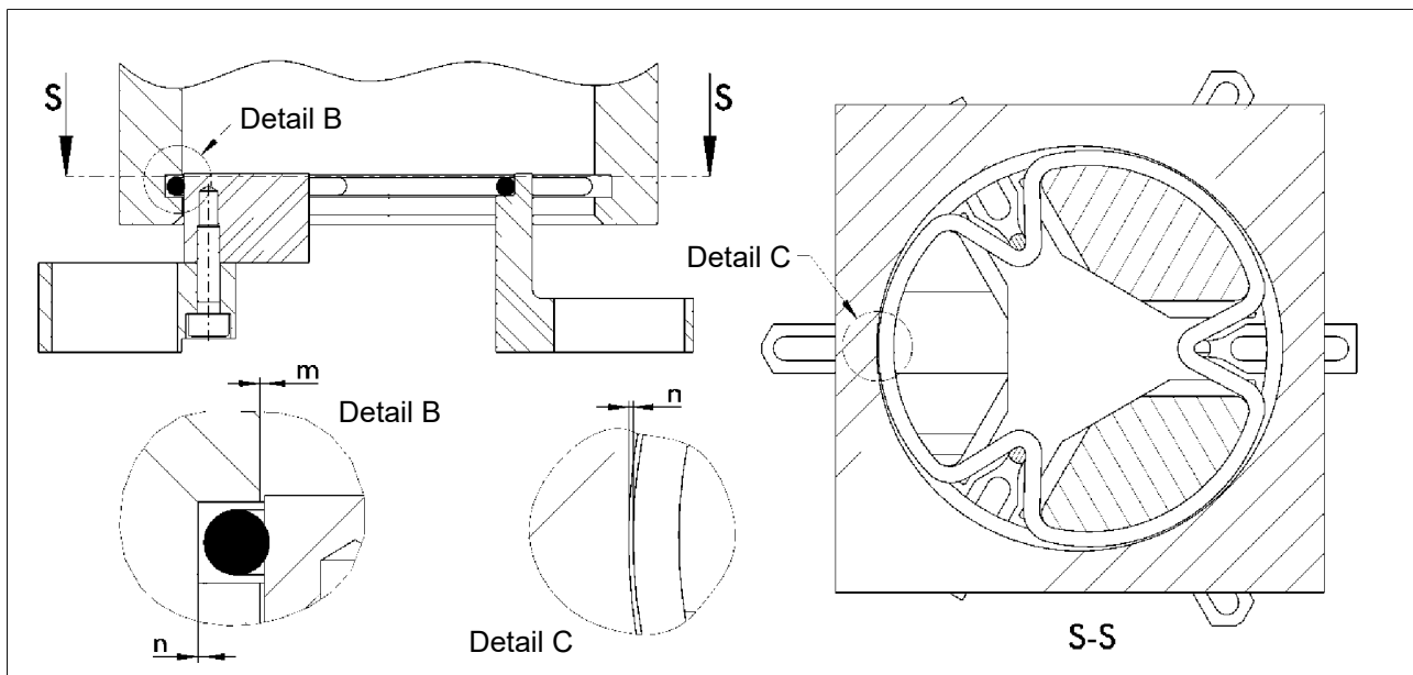
Setting triple jaw B stroke
