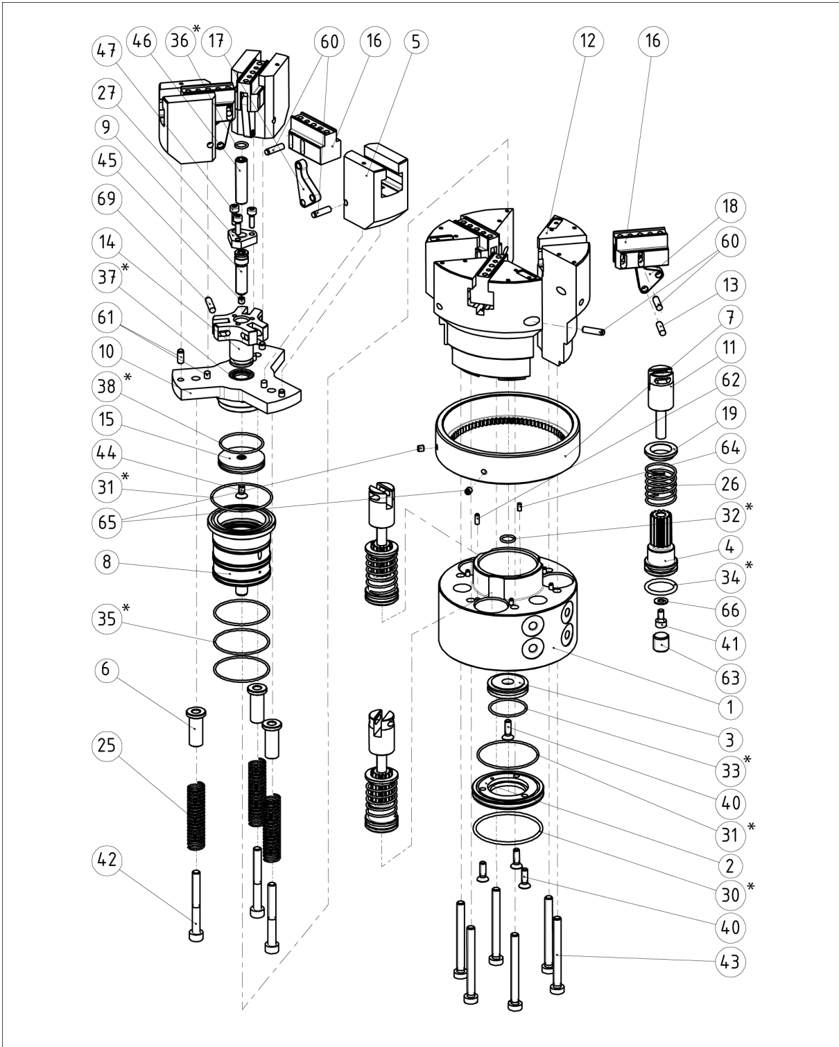
Exploded view ORG 85
