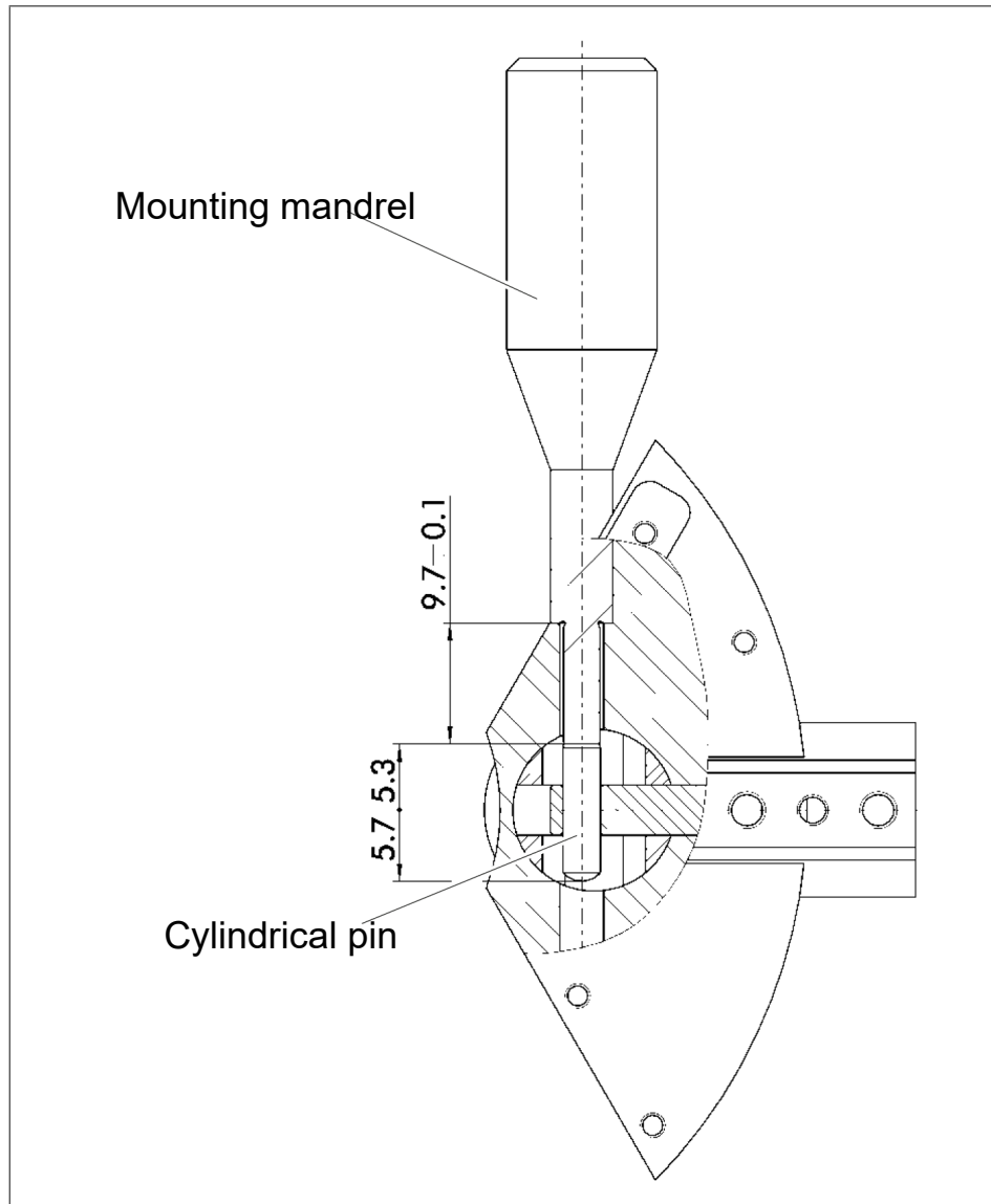
Assembly of cylindrical pins (13)
