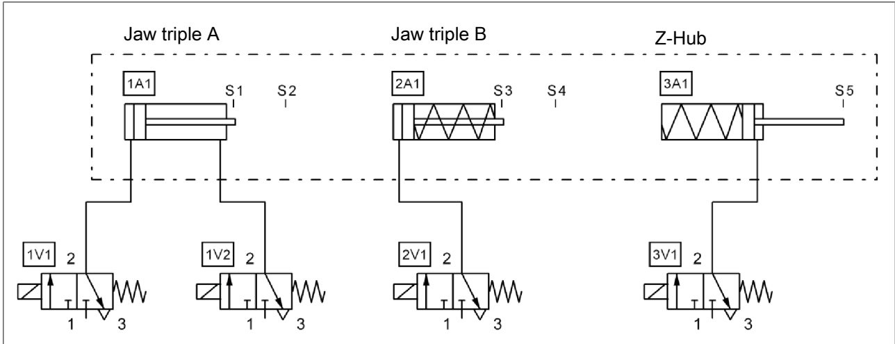
Pneumatic circuit diagram for ORG with four 3/2-way valves
