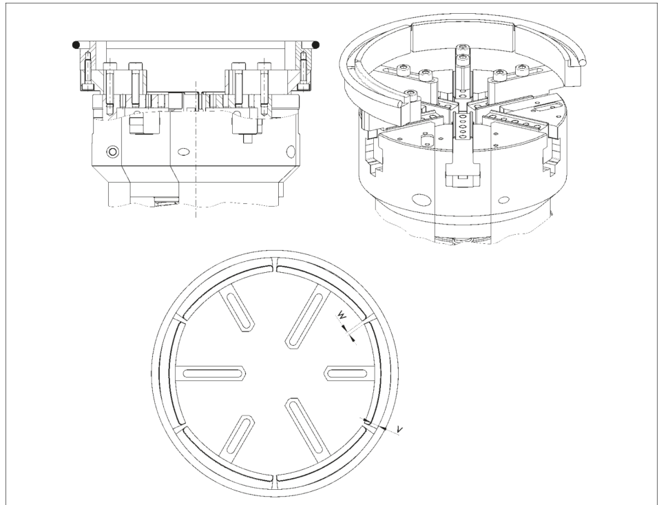
External assembly AM_2.1, Range of inside seal diameter between d_1 > 60 mm and approx. d_1 = 150 mm
