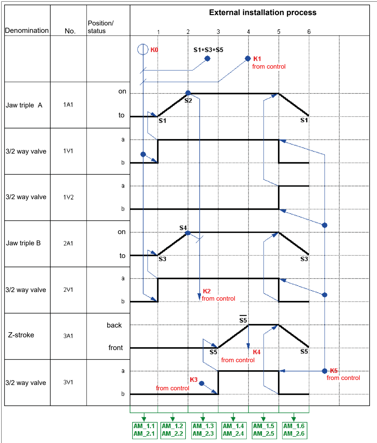
Function diagram external assembly
