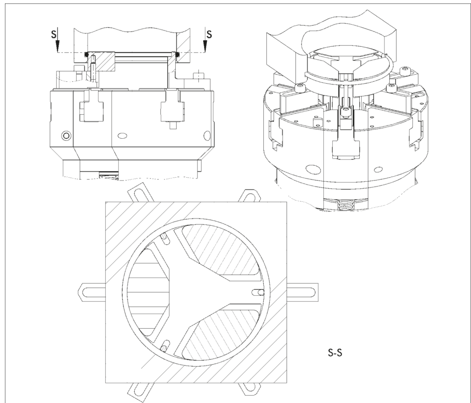
Internal assembly IM_1.9
