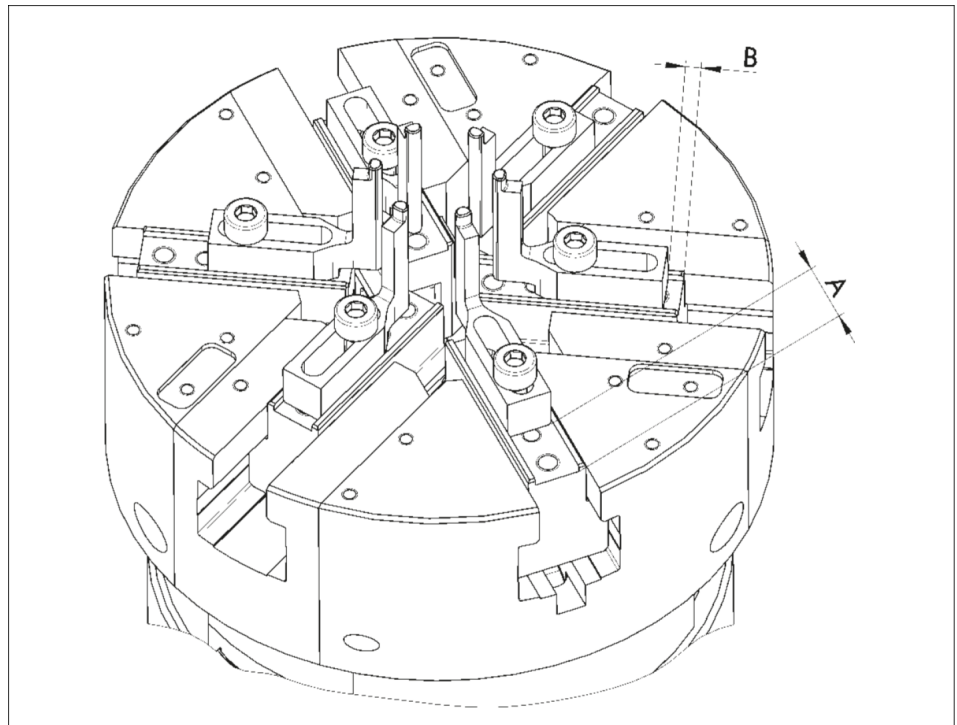
Distance between gripper finger and base jaw
