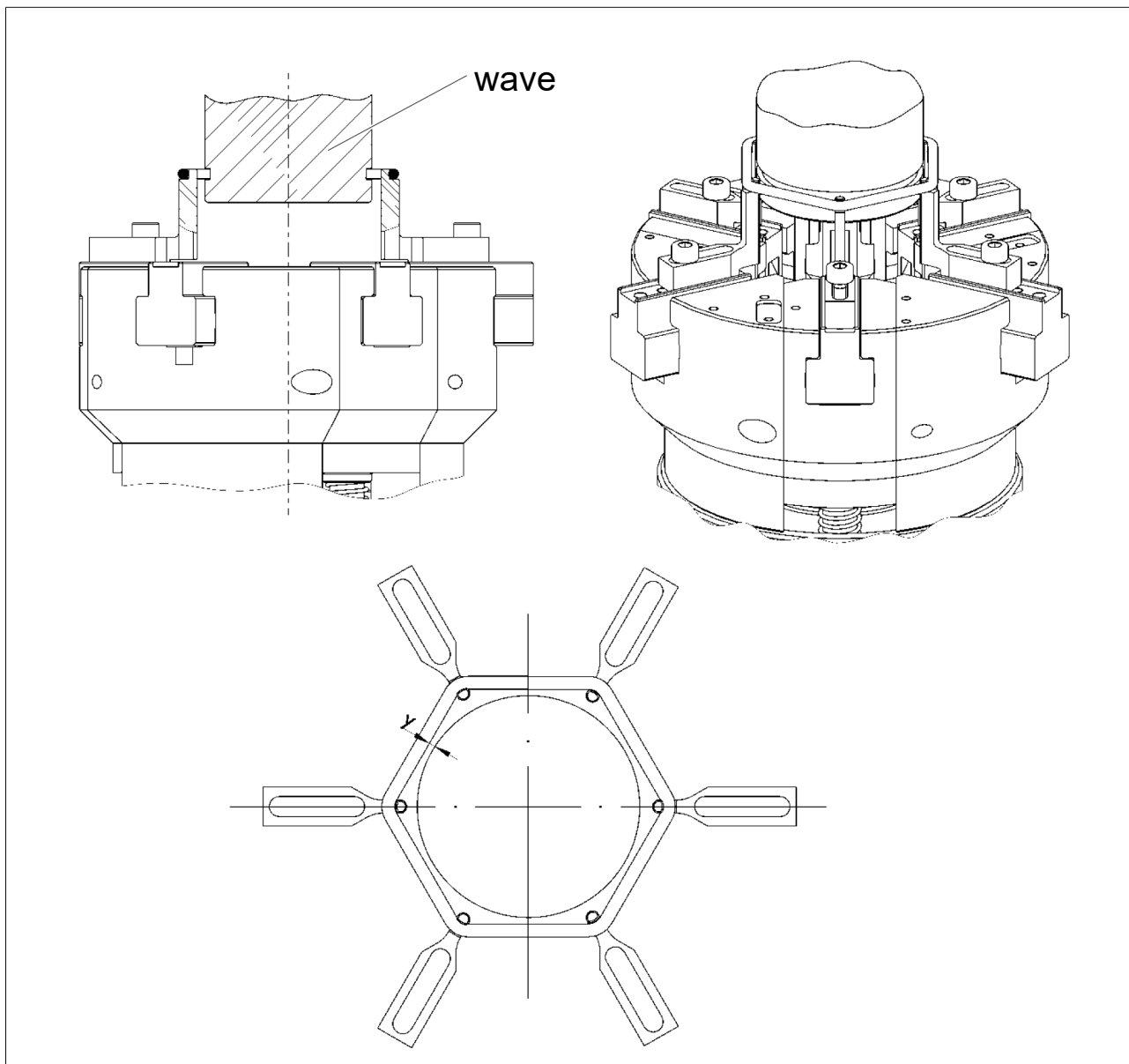
External assembly AM_1.3, Range of inside seal diameter between d_1=10 mm and d_1=60 mm
