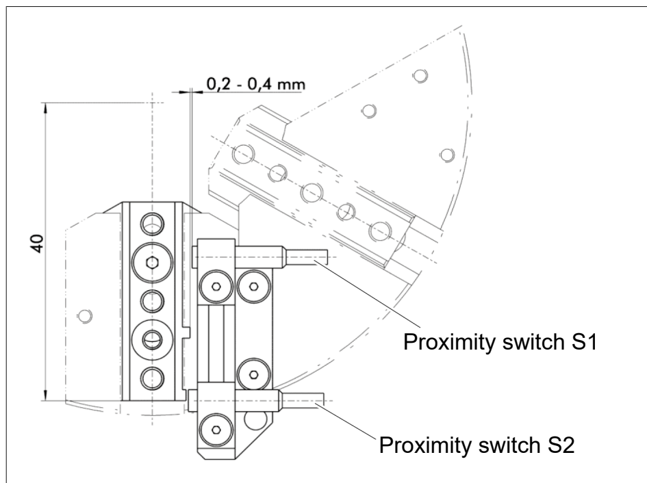
Step 3 Setting proximity switch
