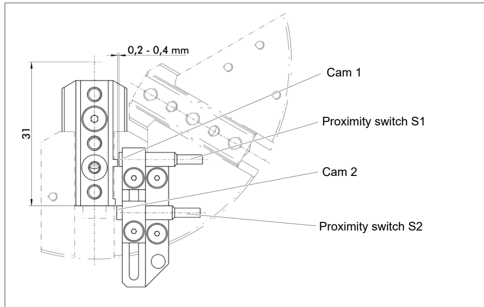
Step 1 Setting the proximity switches
