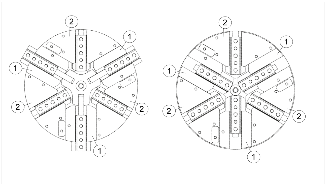
Left: Triple jaw A "open" and triple jaw B "closed"; Right: Triple jaw A and B closed (gripper closed)
