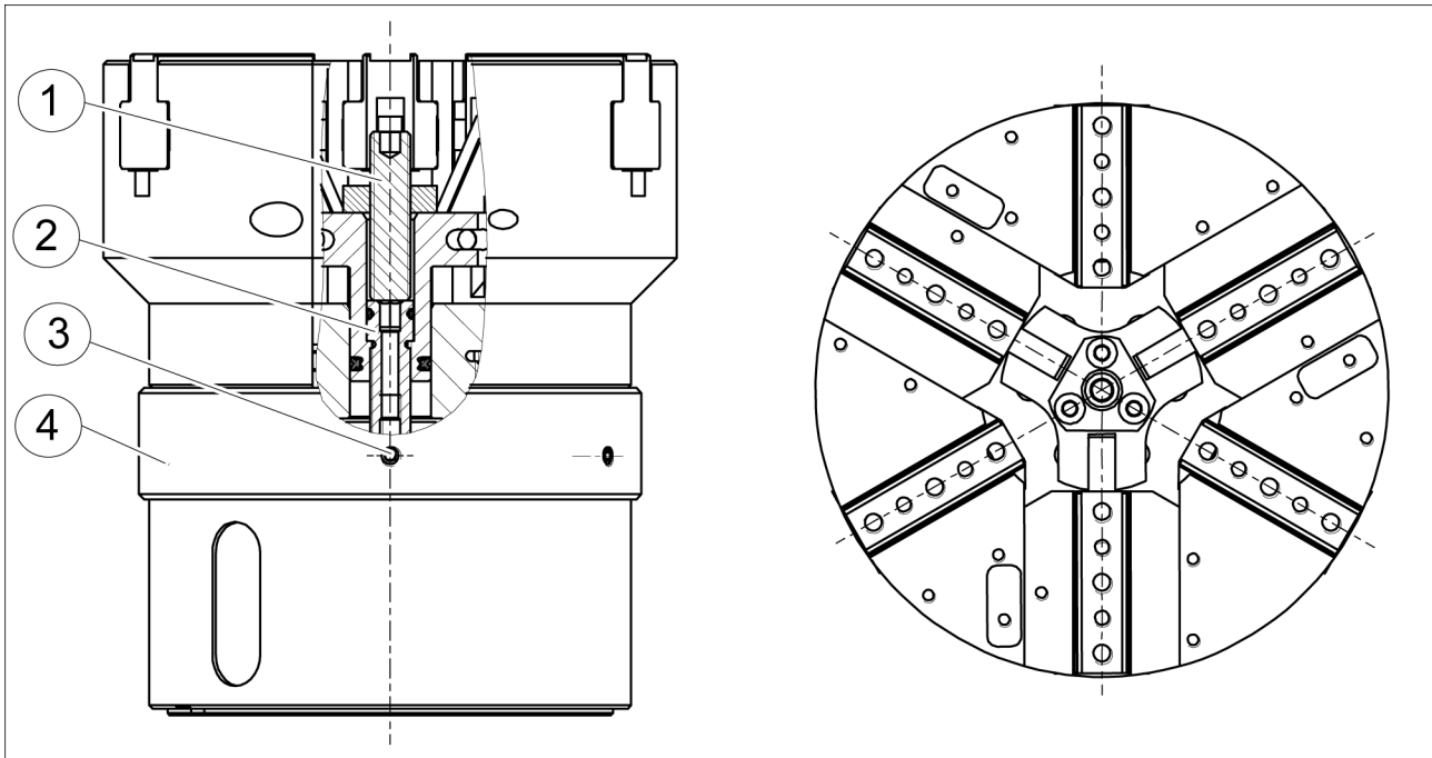
Setting the end positions
