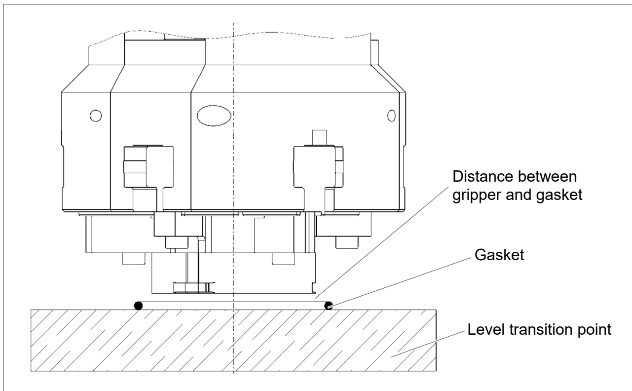
Internal assembly IM_1.1
