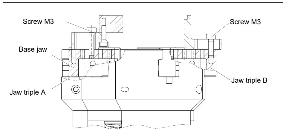
Fastening of gripper fingers and segment jaws with clamping jaws for internal assembly
