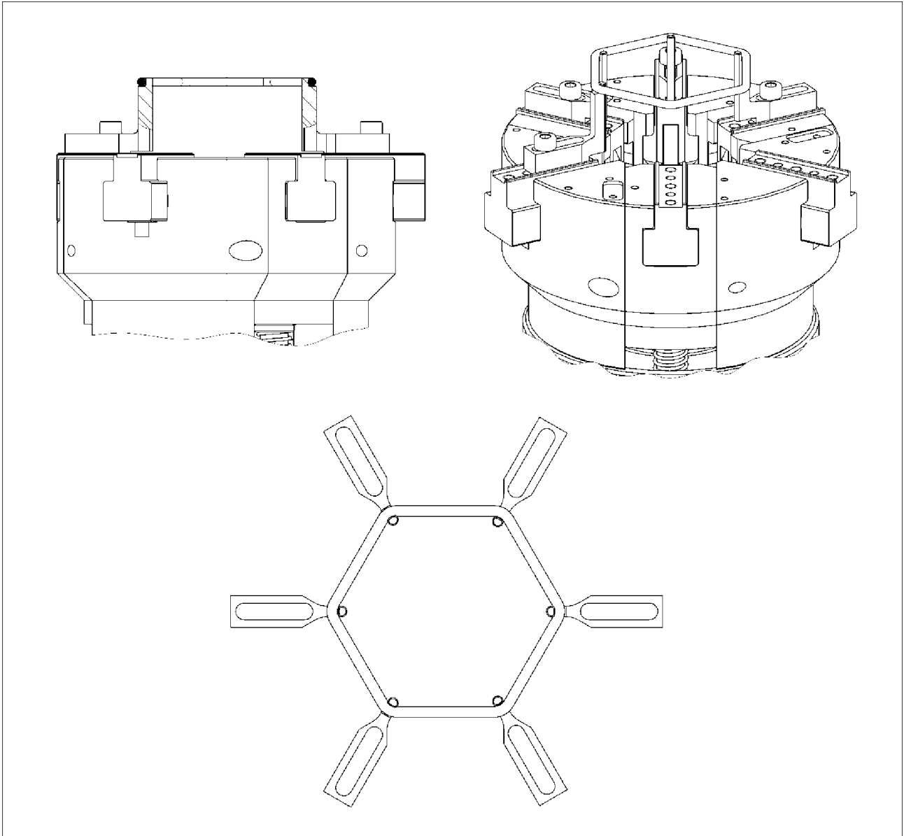
External assembly AM_1.2, Range of inside seal diameter between d_1=10 mm and d_1=60 mm
