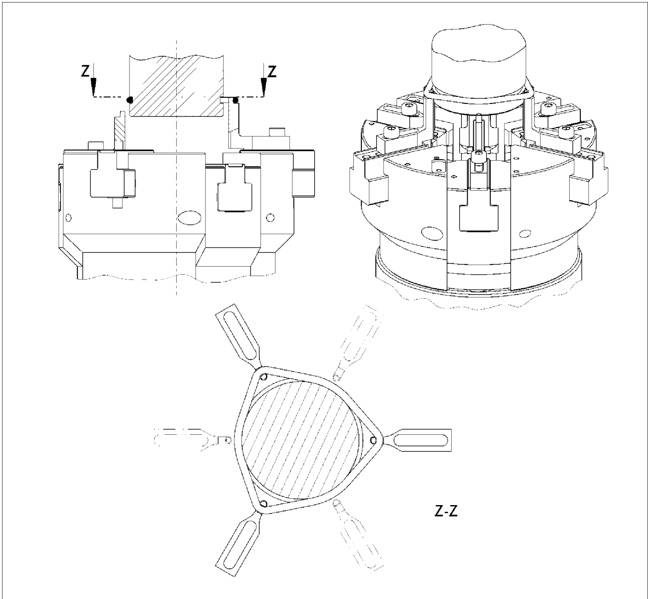
External assembly AM_1.4, Range of inside seal diameter between d_1=10 mm and d_1=60 mm
