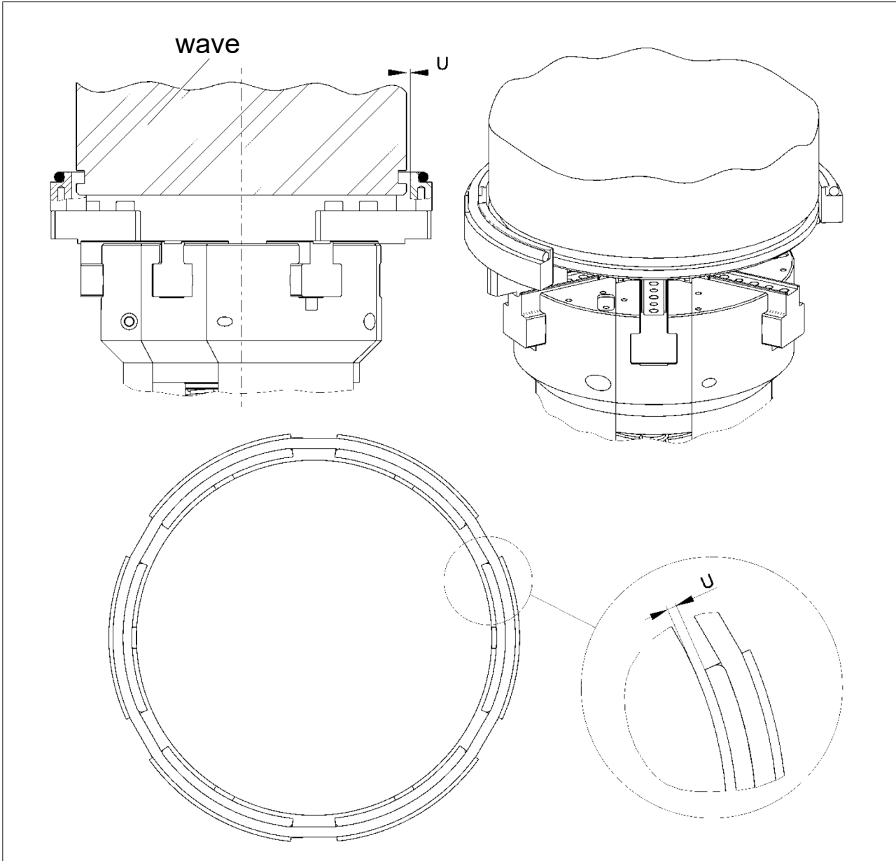
External assembly AM_2.3, Range of inside seal diameter between d_i > 60 mm and approx. d_i = 150 mm
