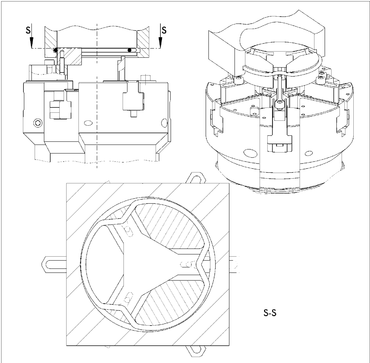
Internal assembly IM_1.7
