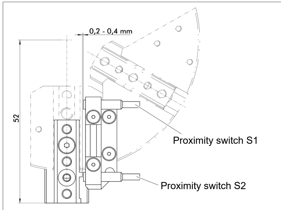
Step 6 Setting the proximity switches
