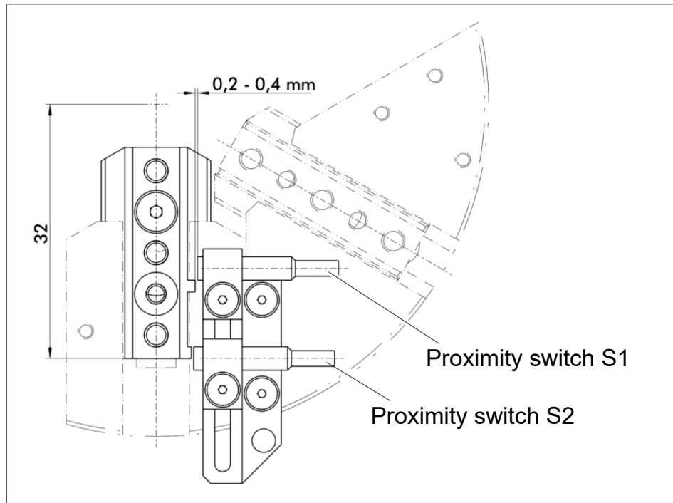
Step 2 Setting the proximity switches
