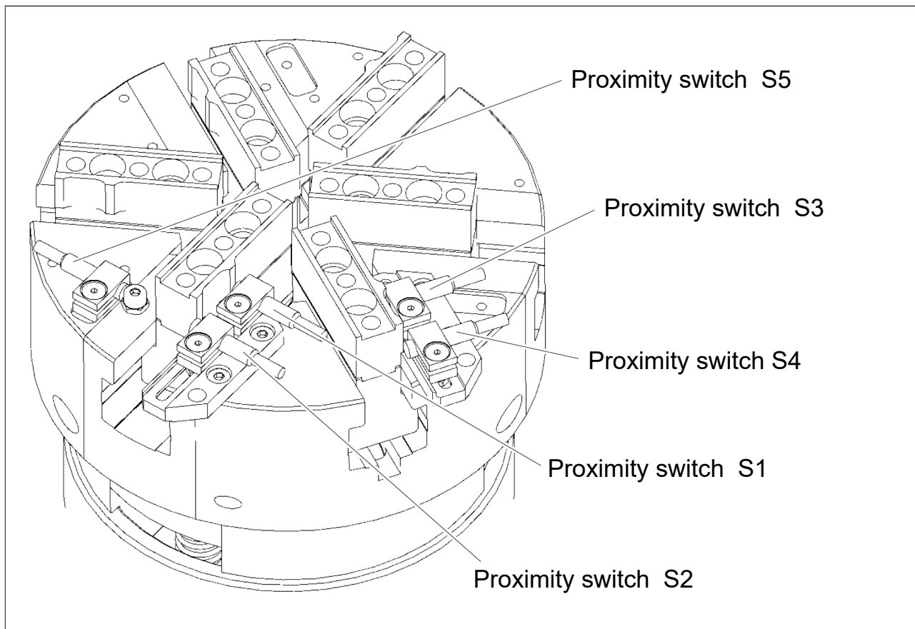
Overview of proximity switches on the gripper
