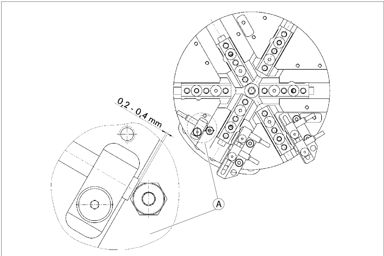
Z-stroke monitoring
