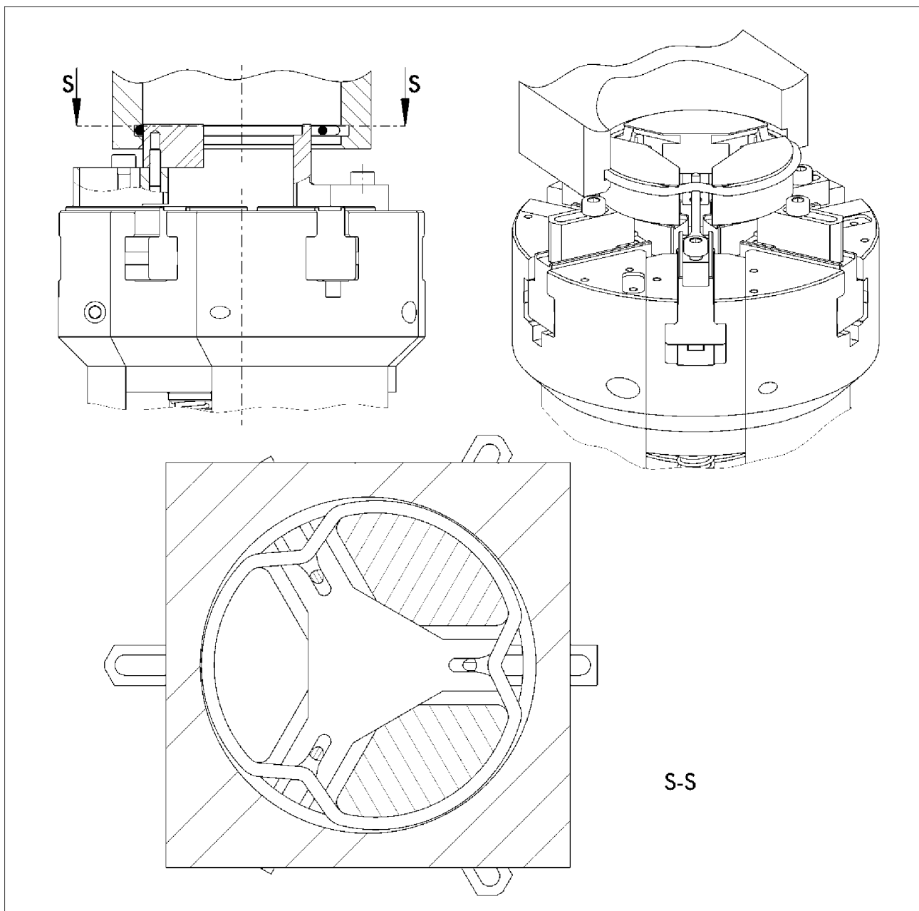
Internal assembly IM_1.8
