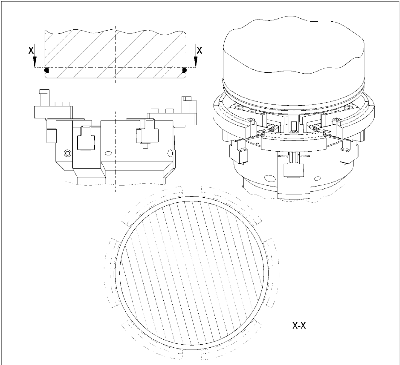
External assembly AM_2.5, Range of inside seal diameter between d_i > 60 mm and approx. d_i = 150 mm
