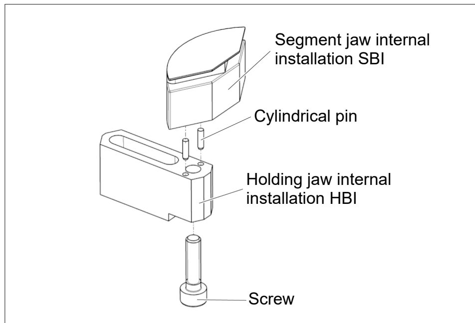
Installation of segment and clamping jaw for internal assembly
