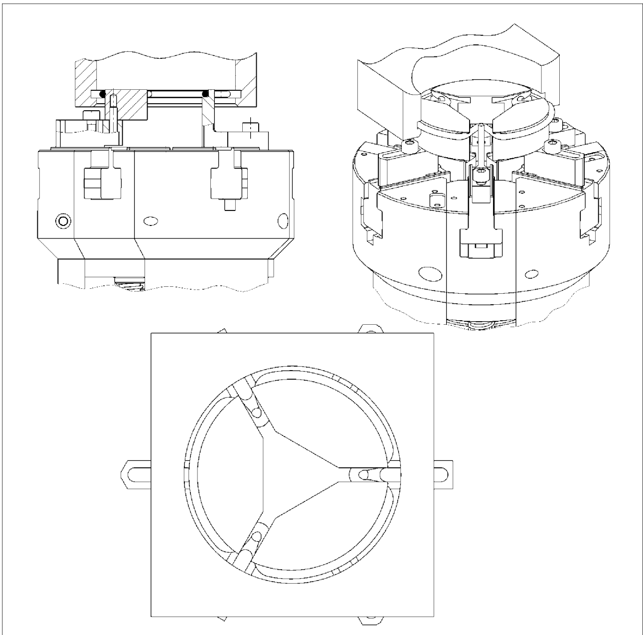
Internal assembly IM_1.5
