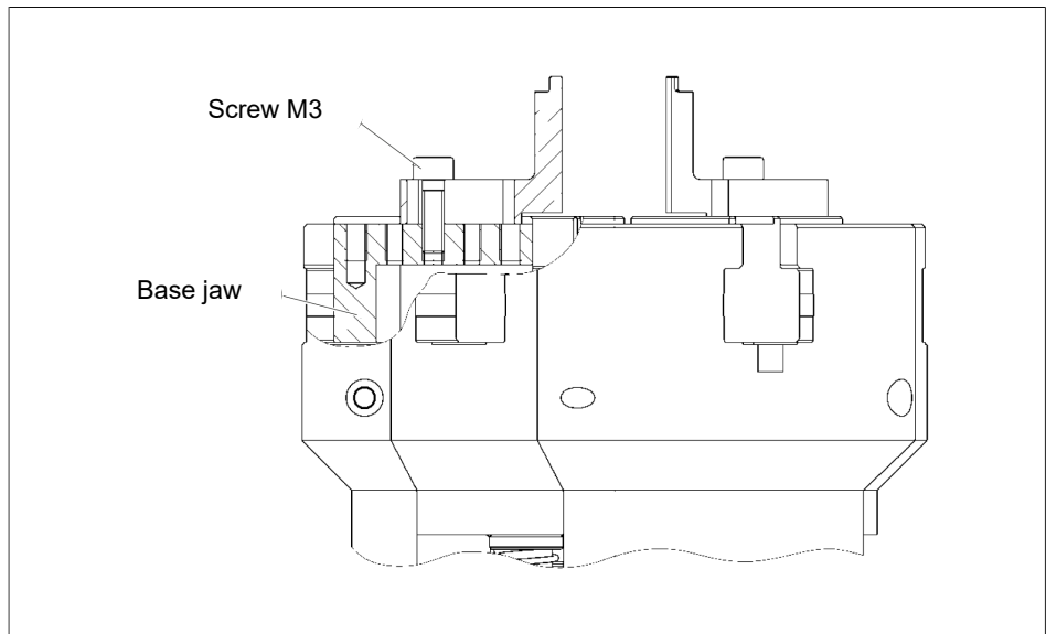
Mounting gripper finger external assembly; inner seal diameter between d1=10 mm and d1=60 mm
