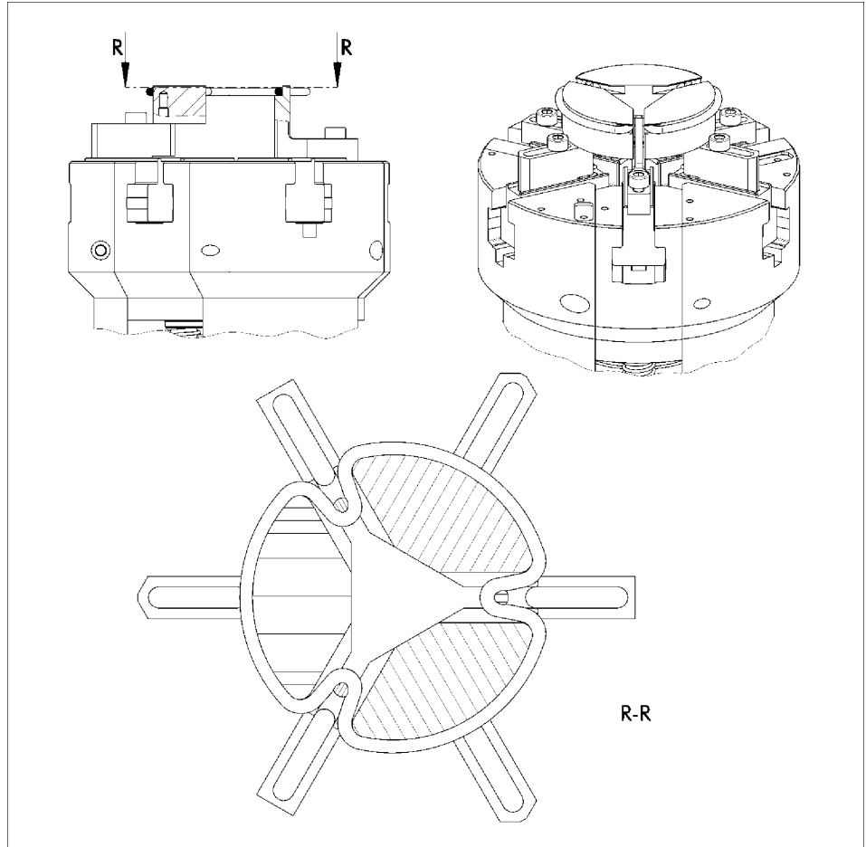
Internal assembly IM_1.4
