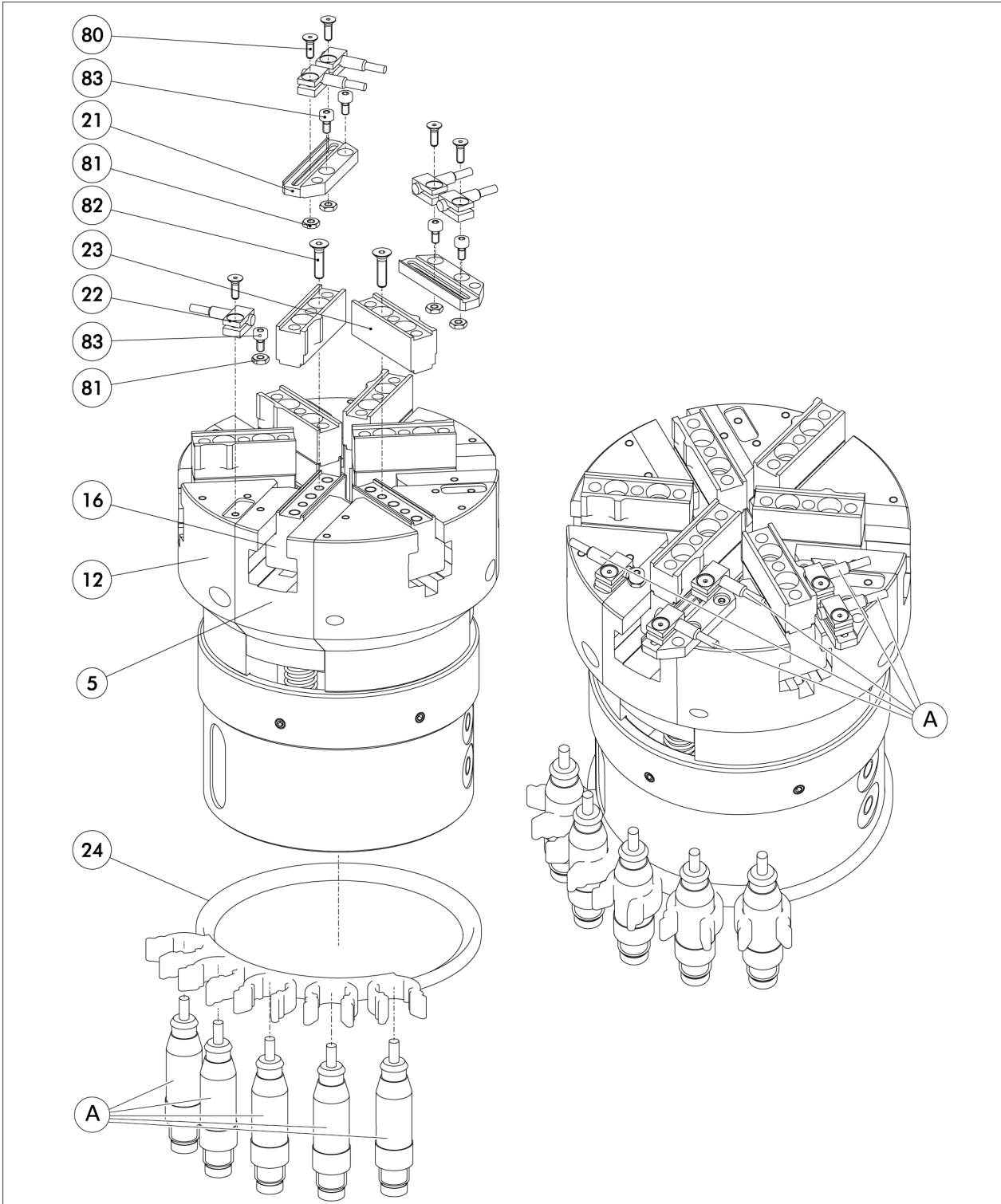
Assembly drawing mounting kit
