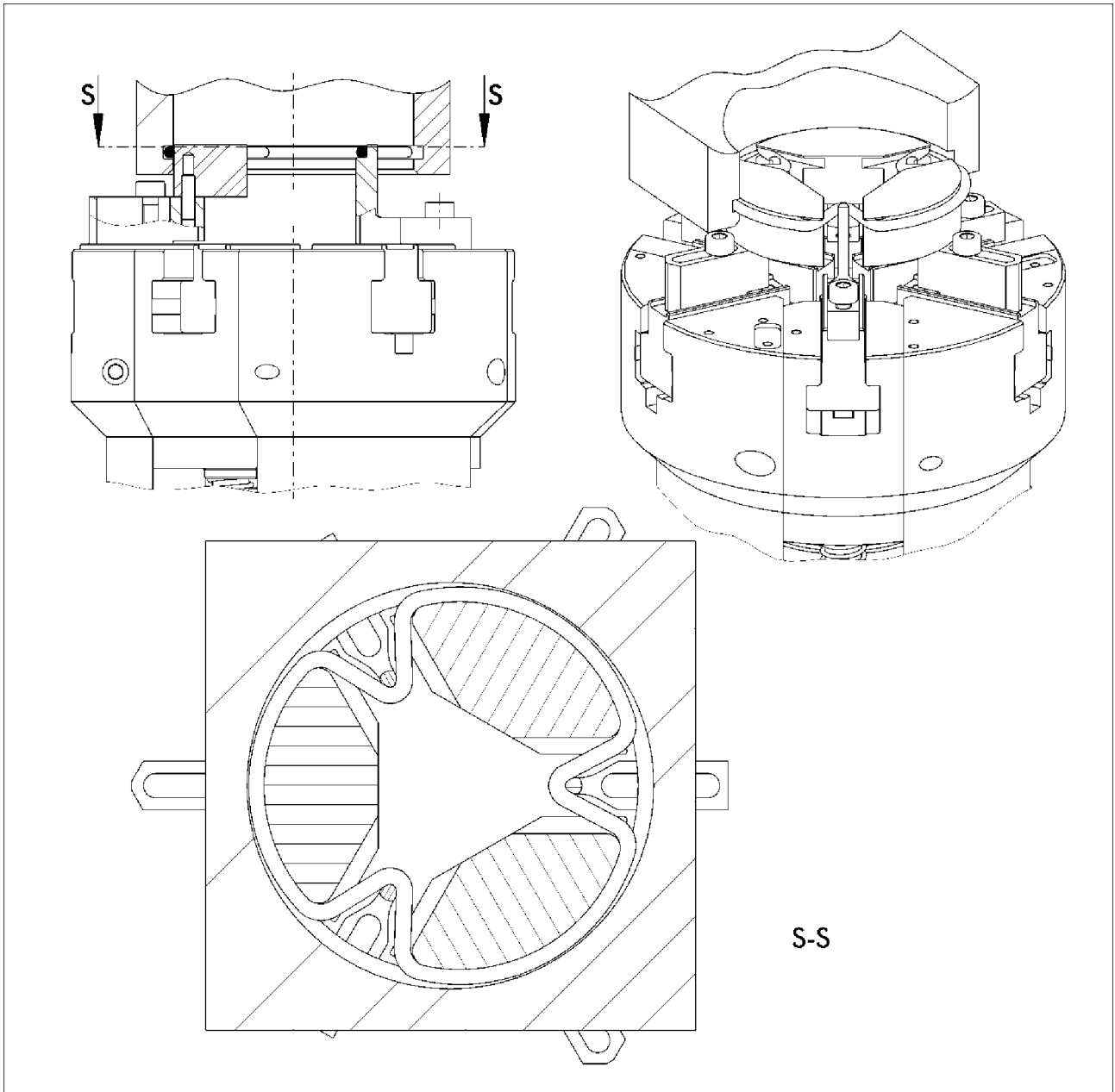
Internal assembly IM_1.6
