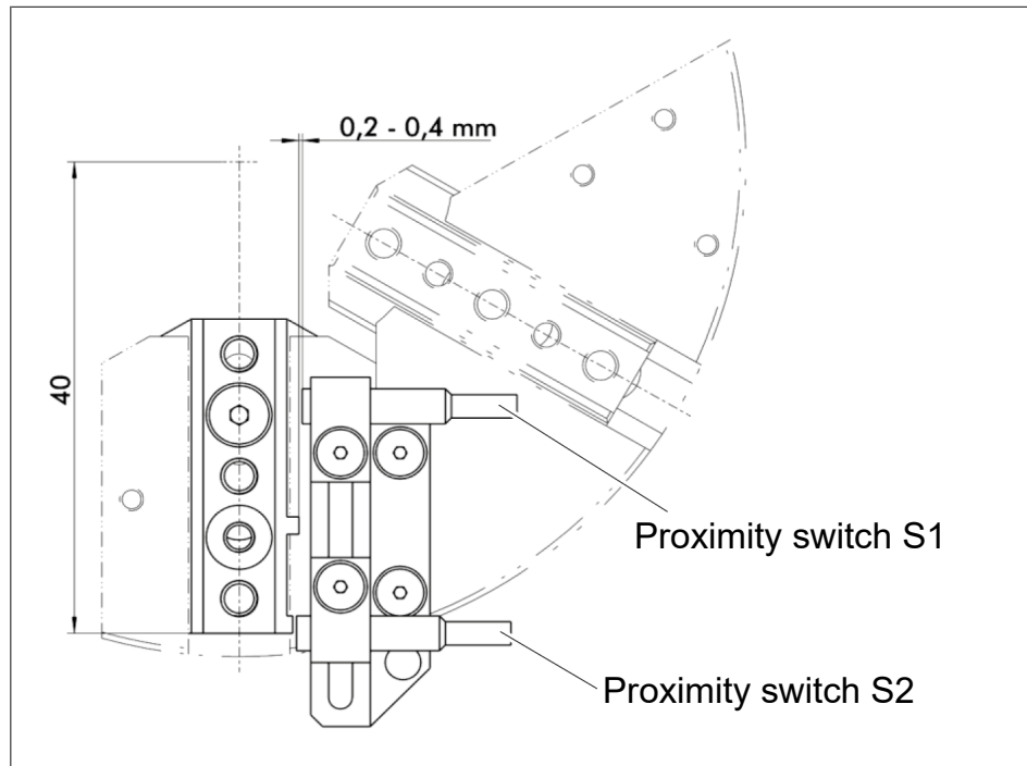
Step 4 Setting the proximity switches
