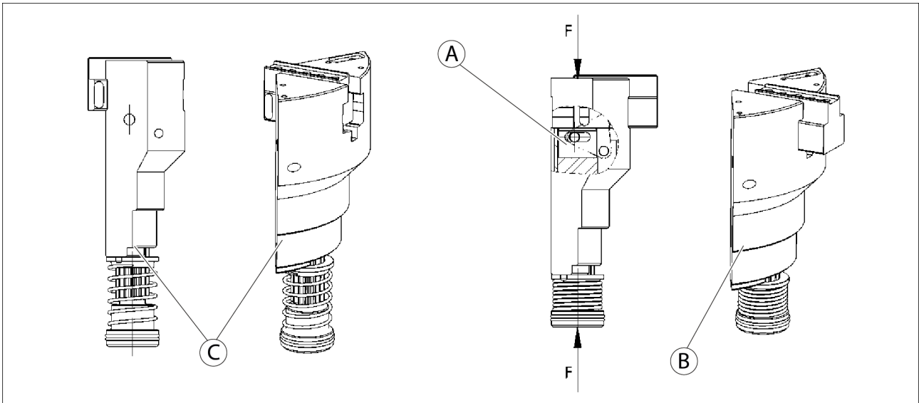
Disassembly of base body with drive unit triple jaw B
