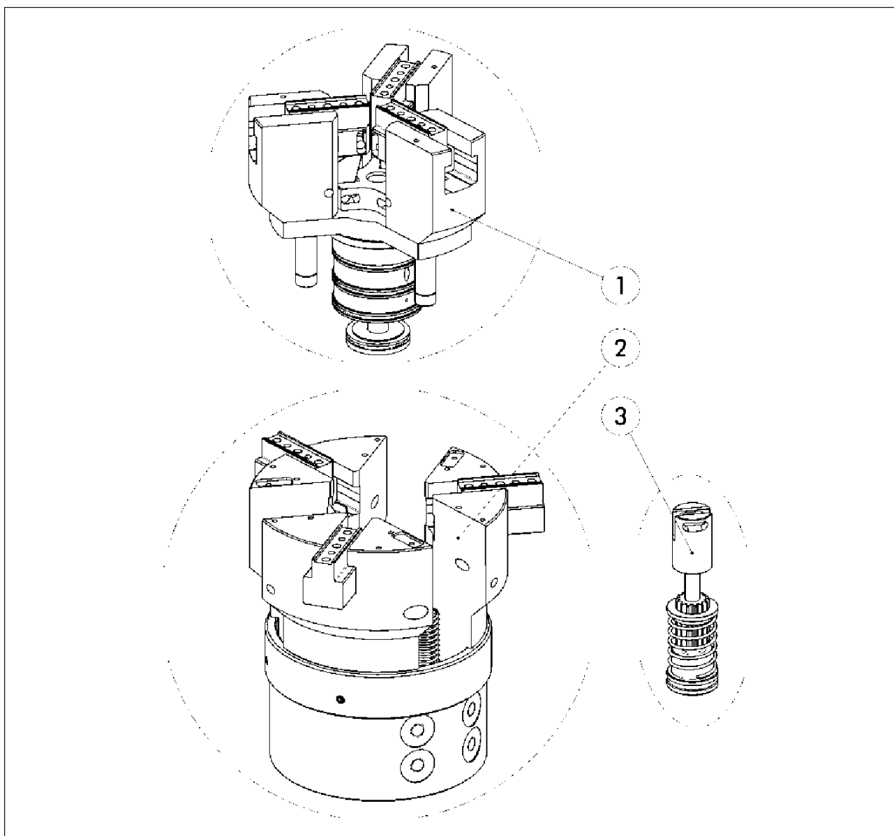
Gripper design
