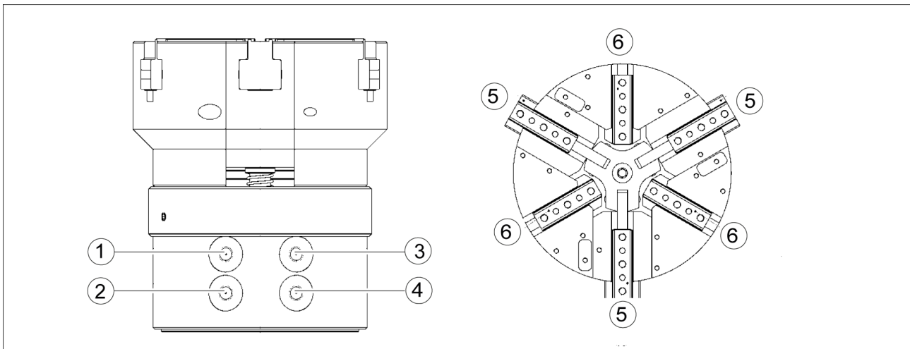
Definition of air connections and triple jaws
