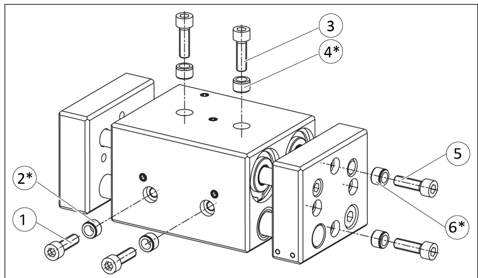
Possible assemblies, metric version
