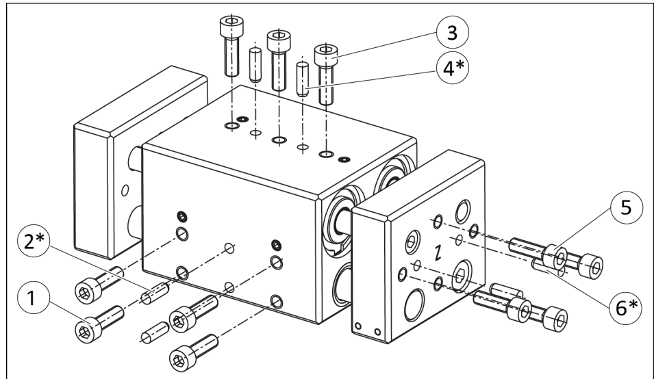
Possible assemblies, inch version
