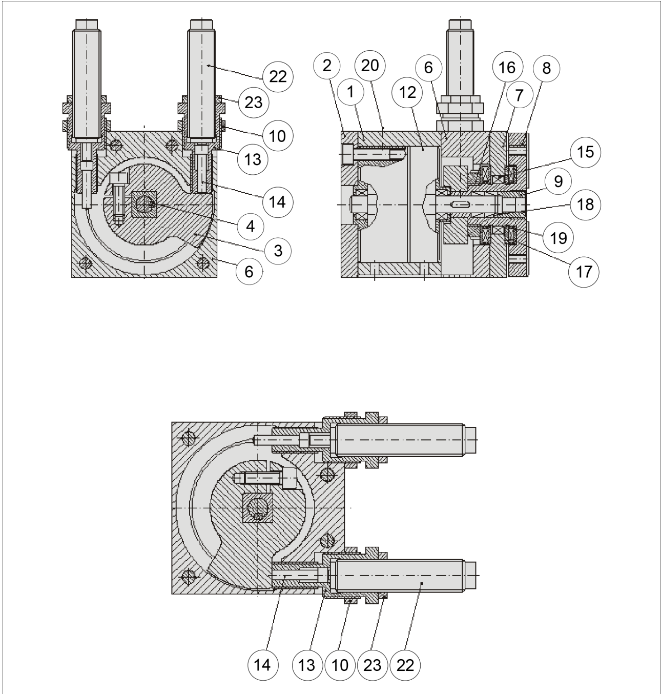
Assembly of RM 06
