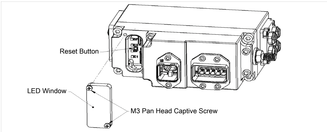
Reset Button
