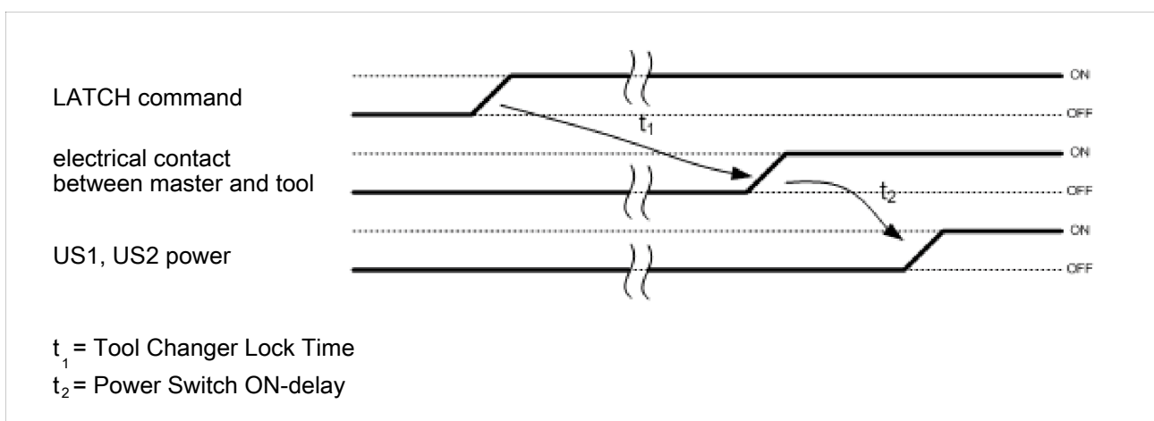
Power-On Timing
