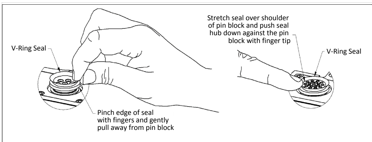
V-Ring seal Replacement
