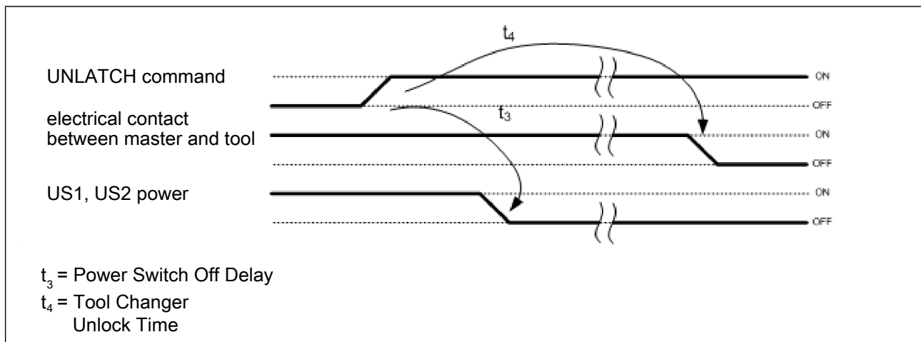
Arc Prevention Circuit Power-Off Timing
