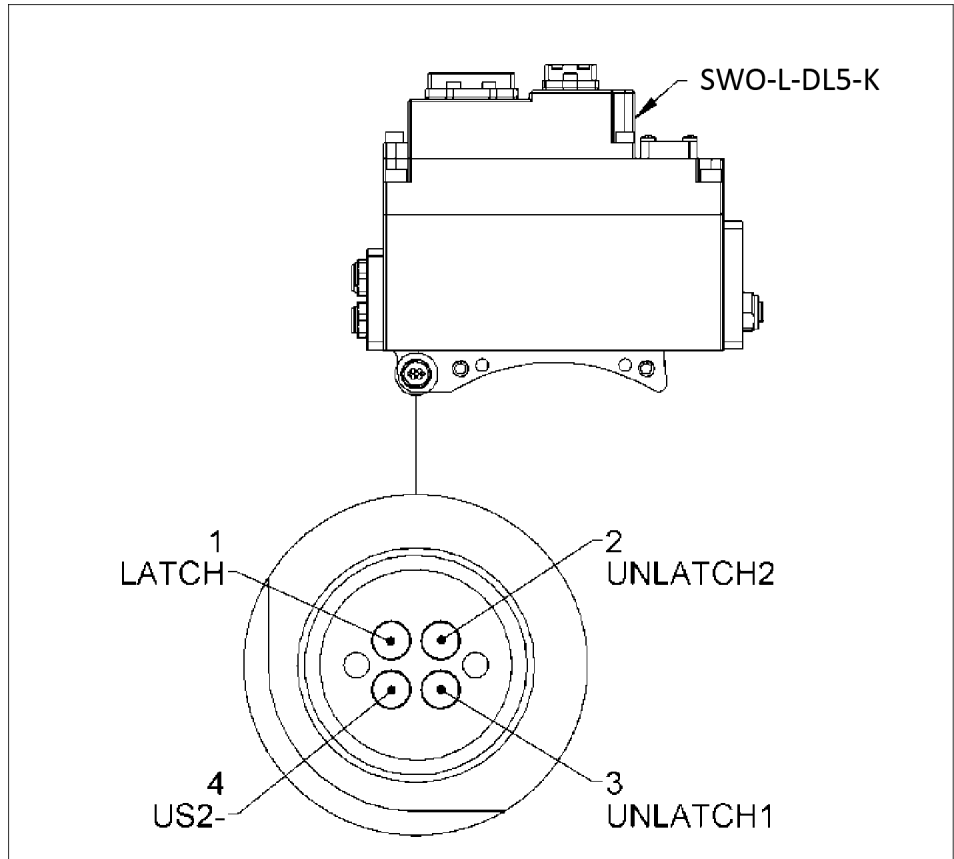
Pin Internal Pin Block
