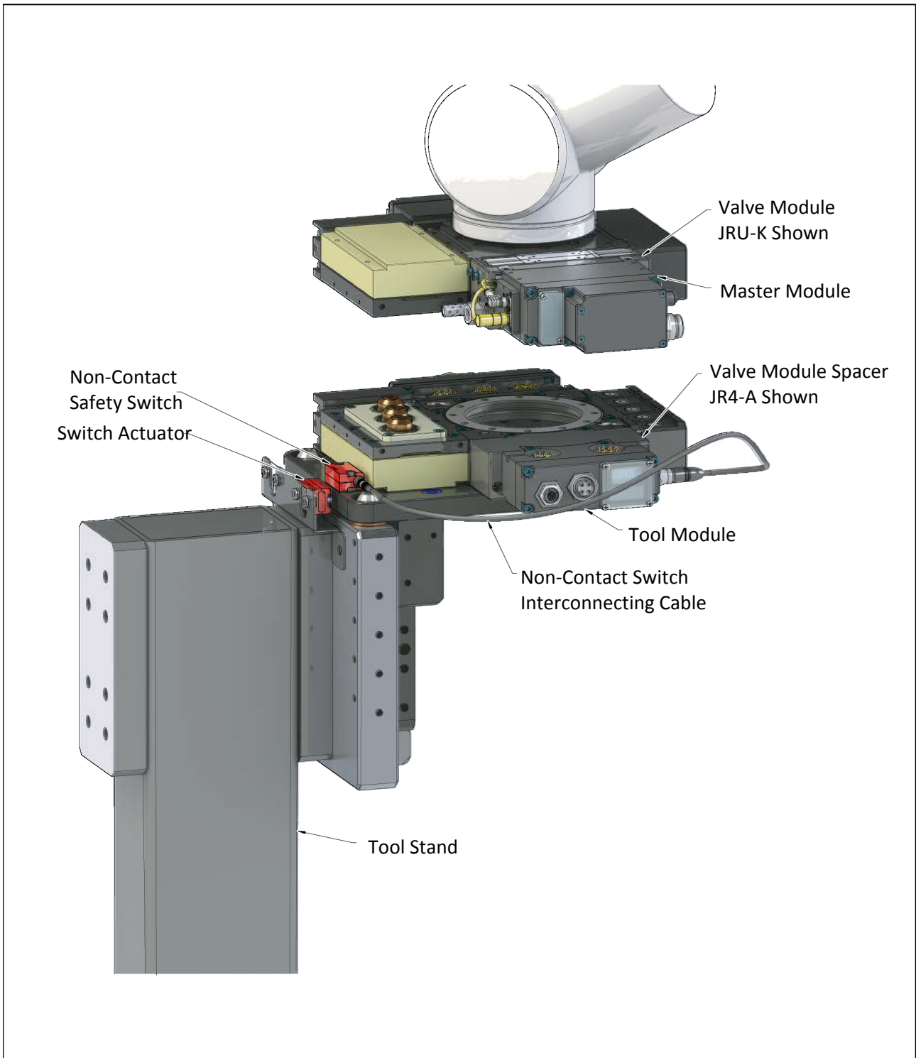
Safety Switch (Modules Shown for Reference Only)
