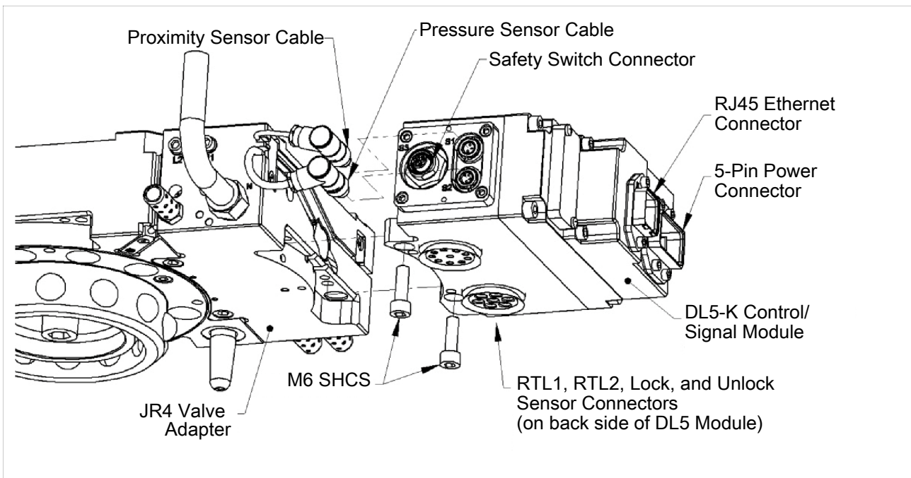
Module Installation and Removal DL5-M Control/Signal Module
