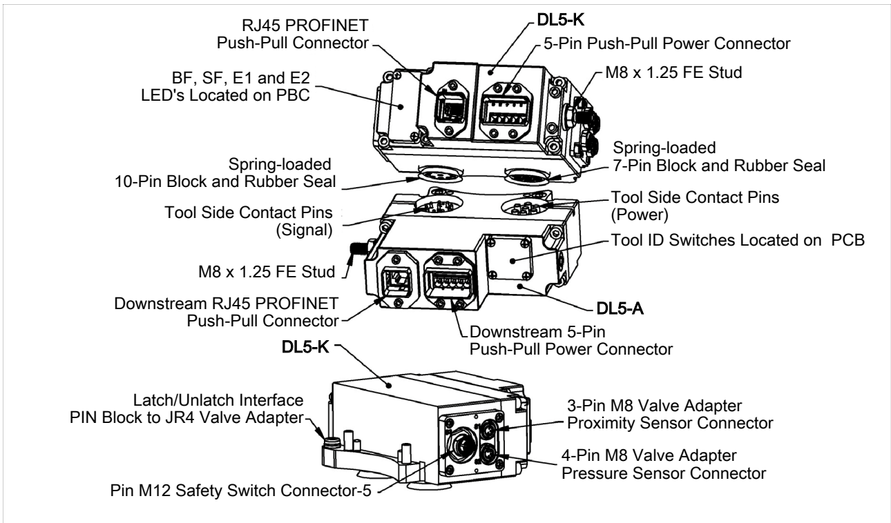
DL5 PROFINET Master and Tool Modules
