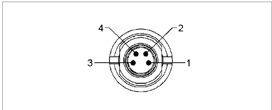
M8 4-Pin Female Valve Adapter Pressure Sensor
