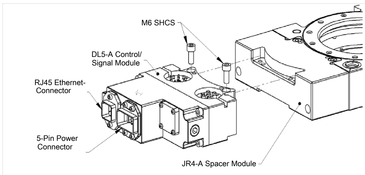
Module Installation and Removal DL5-T Control/Signal Module
