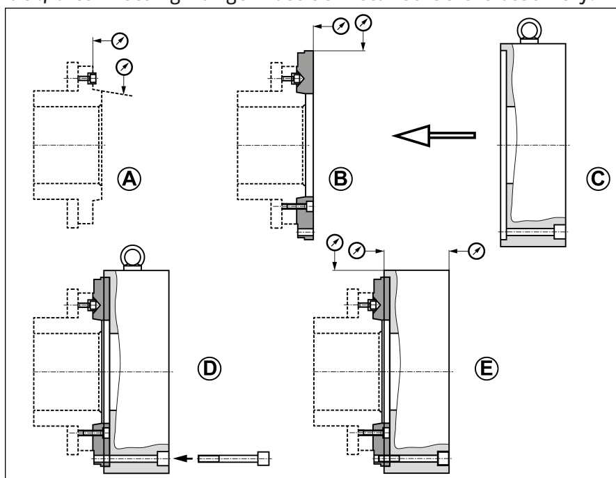
Chuck assembly
