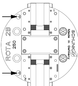
Fig. 1: Lubricating points
