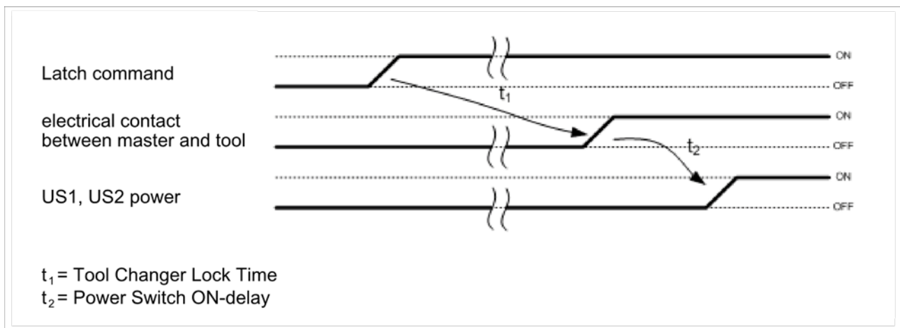
Power-On Timing
