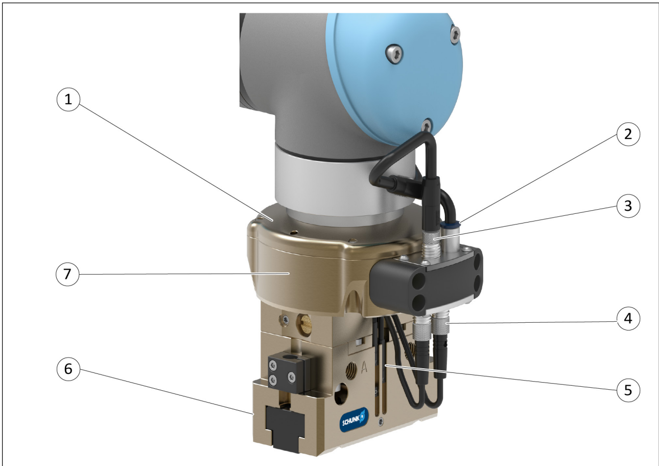
JGP 100 with adapter on robot
