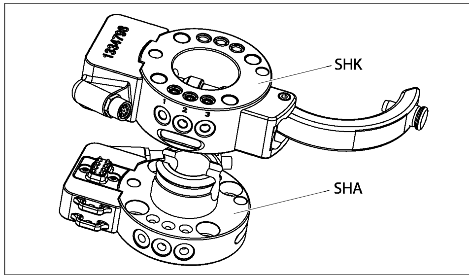
Drilling pattern to DIN ISO 9409-1, principle
