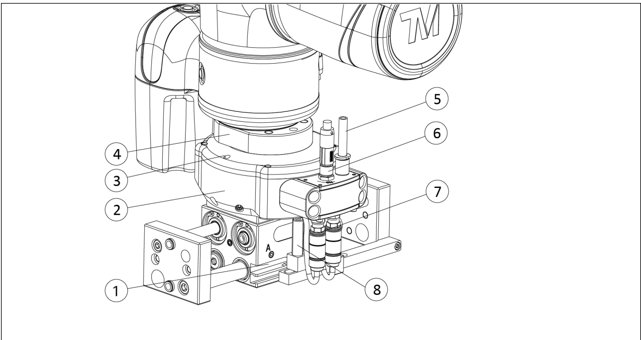
PSH 22-1 with cantilever plate at the robot
