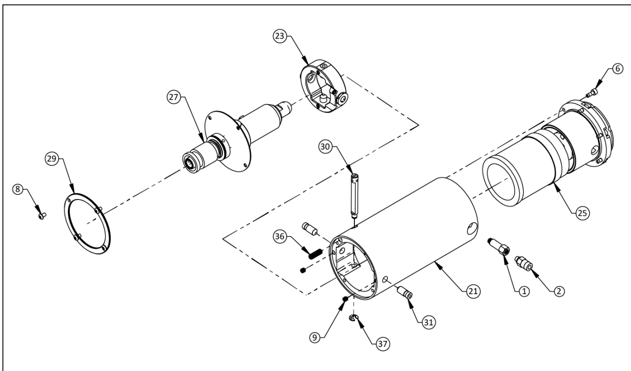
Variant: Manual tool change
