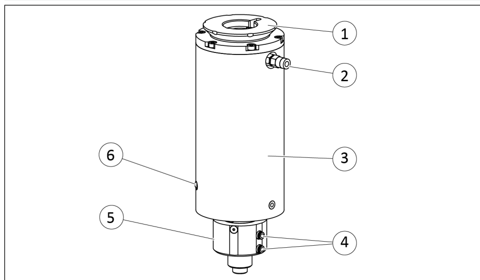
Axially and radially flexible deburring tool with Auto Tool Changer
