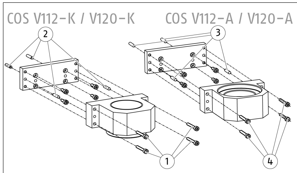
Mounting optional module COS V112, 200
